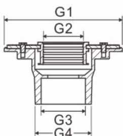
ABS membrane coupling drawing
